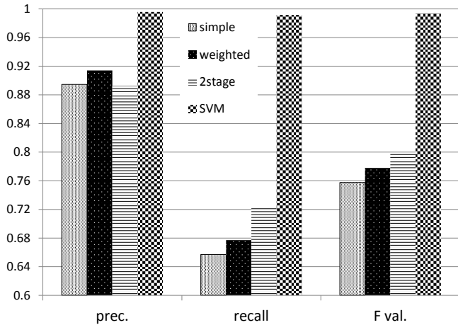
Fig. 4: Closed test (graph)
