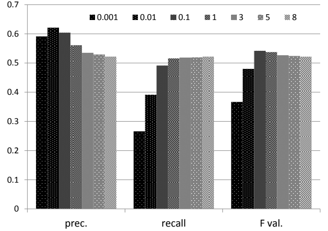
Fig. 5: Slack variable cost and performance (5-fold)
