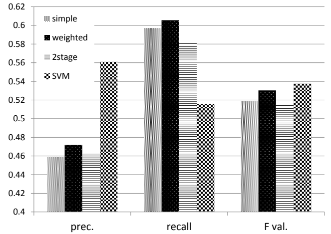
Fig. 2: Simple 5-fold cross validation (graph)
